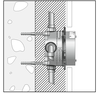
Installation in front of the wall; here with variable spacers on hanger bolts M 10
